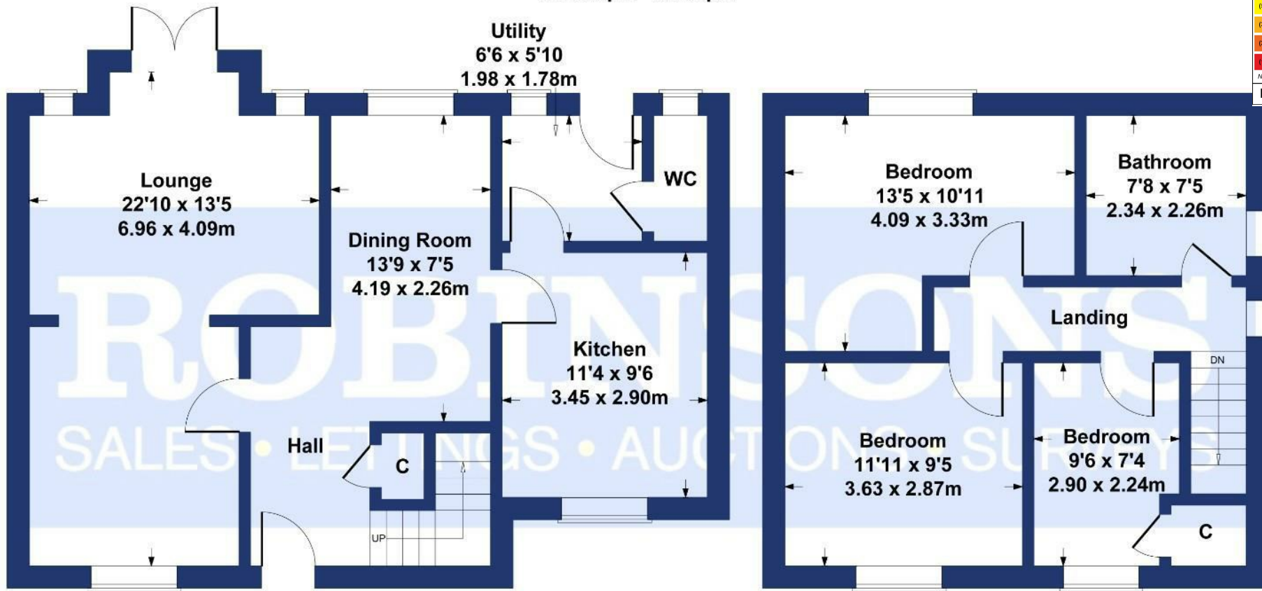
GROUND FLOOR
